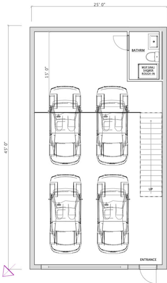
TYPICAL 25 x 45 GARAGE UNIT GROUND LEVEL
