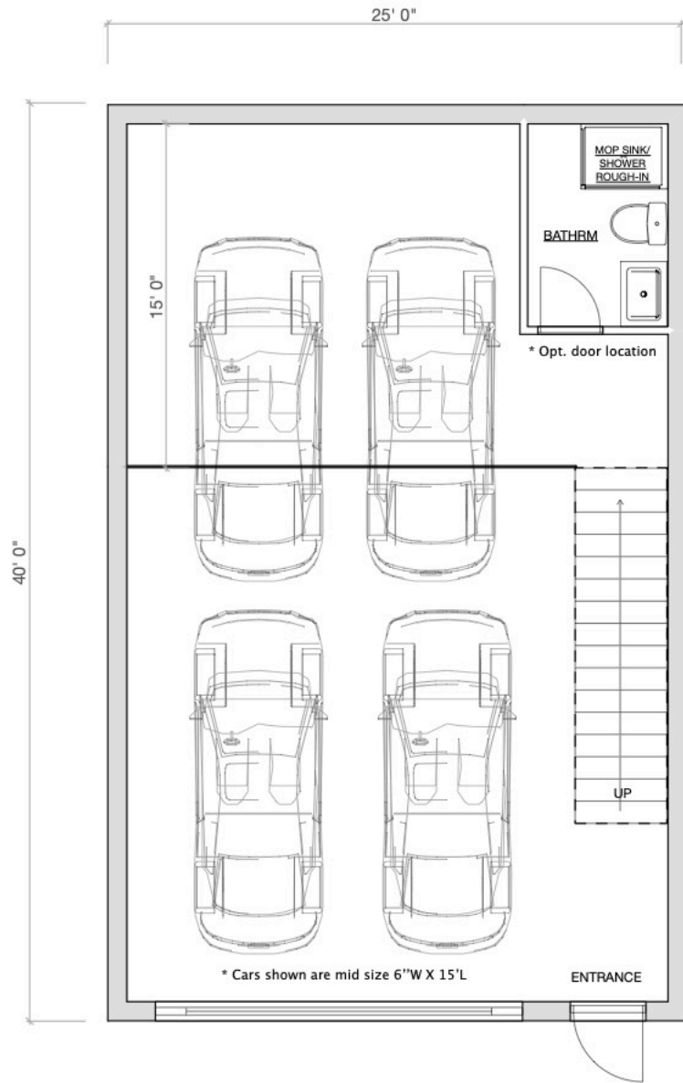
TYPICAL 25 x 40 GARAGE UNIT
